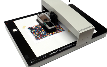
ColorScout A+ for BYKmac
